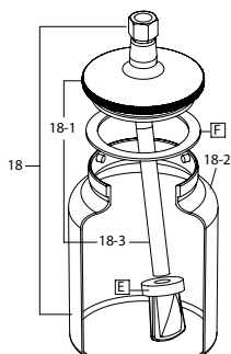
AG-1 - 1L. Pin Lock Cup - (for suction models)
