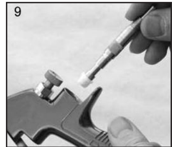
9. Fit New Front Seal to Service Tool so that the groove faces the handle end of tool.
