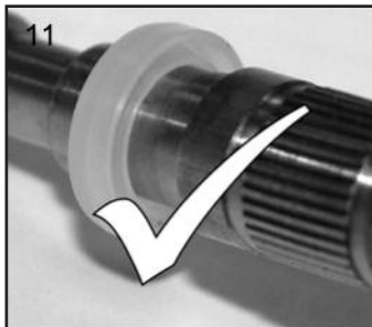
11. Fit New Valve Seat to Service Tool so that the groove faces the handle end of tool.
