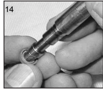
14. Fit new Rear Seal to Service Tool so that the groove faces the handle end of tool.
